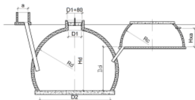
Figure 4: KT1 biogas plant
