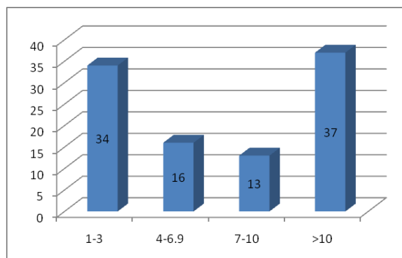
Figure 5: Dillution ratio of biogas digester
